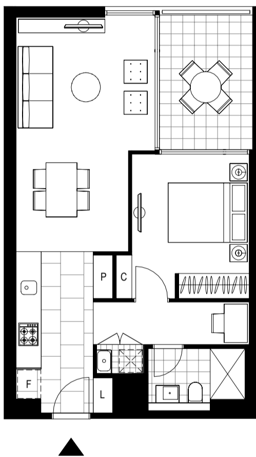
LEVEL 5, 6
